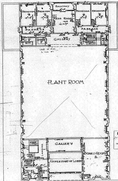
MEZZANINE FLOOR PLAN
