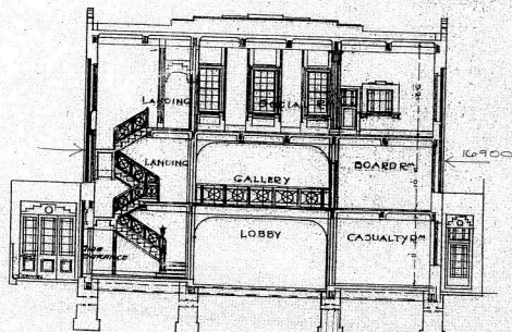
CROSS SECTION C.D.
