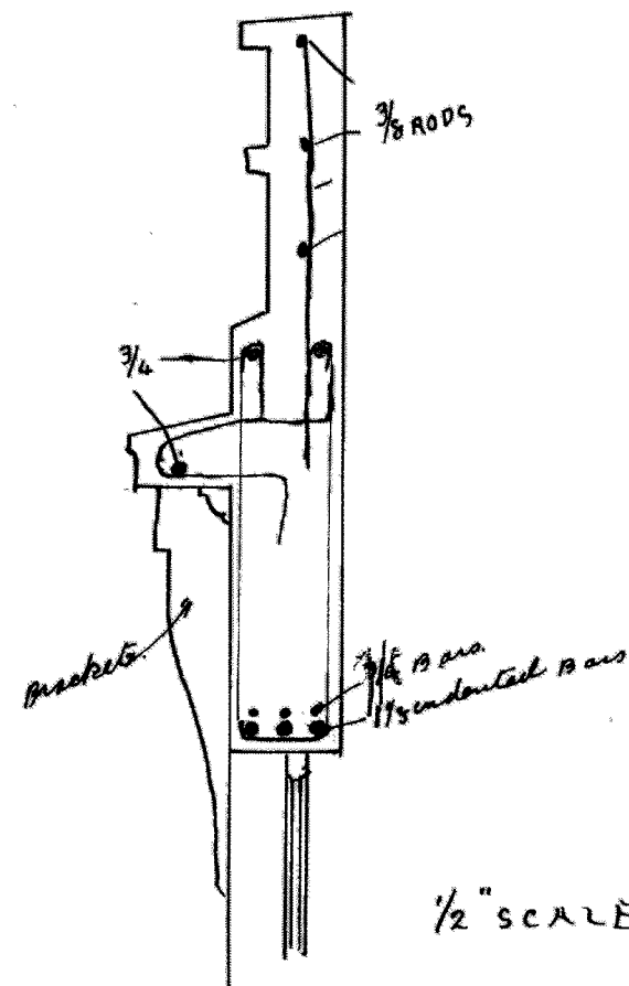
SECTION OF BEAM OVER WINDOWS
