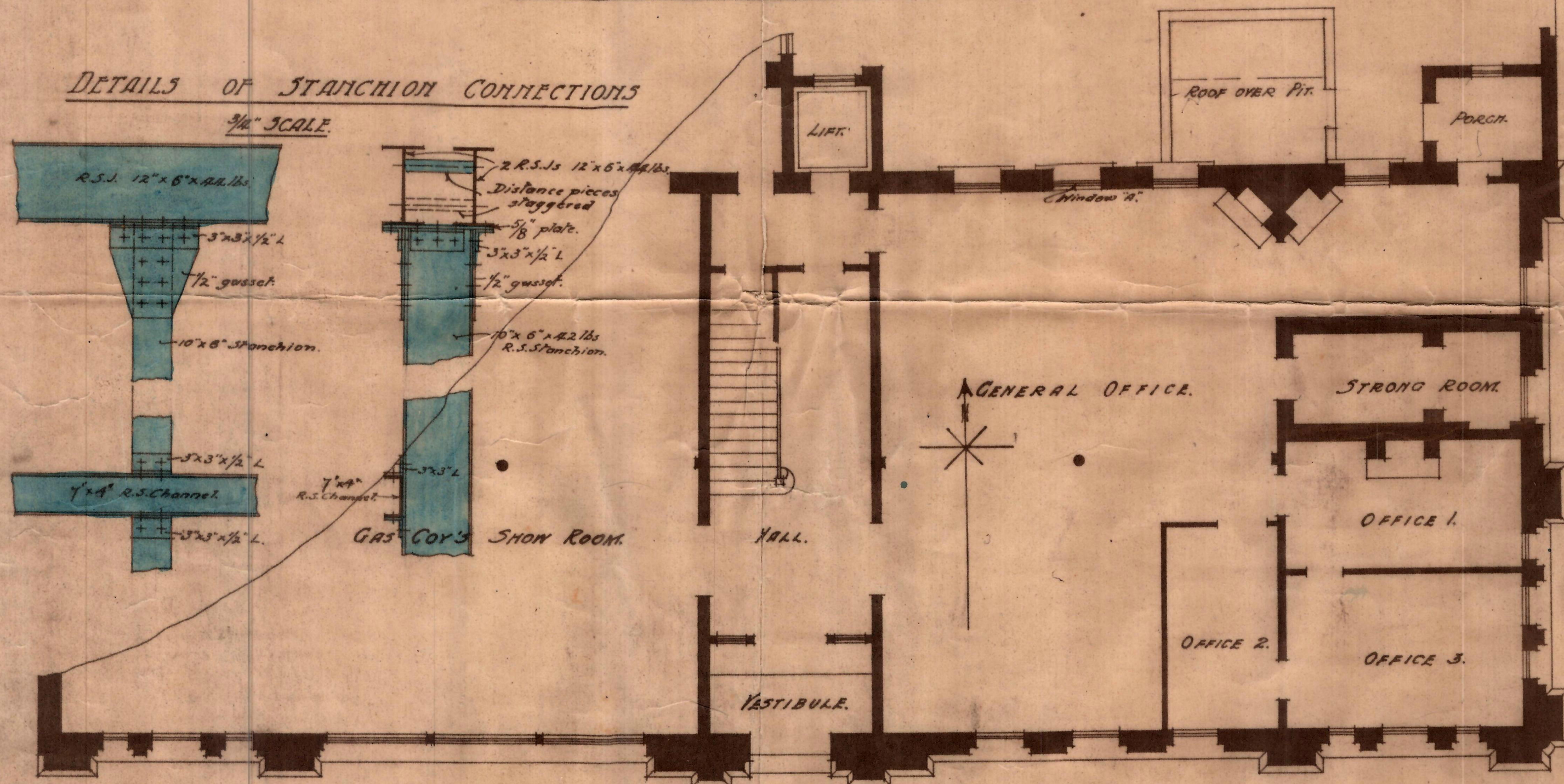
GROUND FLOOR PLAN SHOWING ALTERATIONS.
