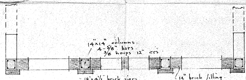
SECTIONAL PLAN.
