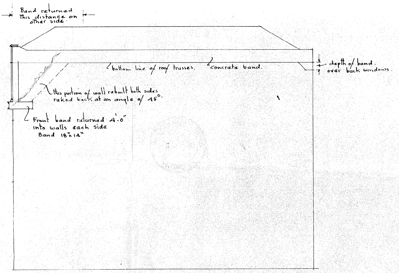
SIDE ELEVATION.
