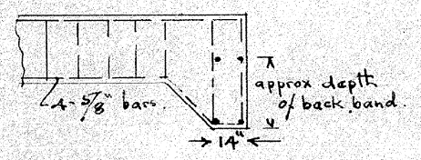
SIDE BAND.
