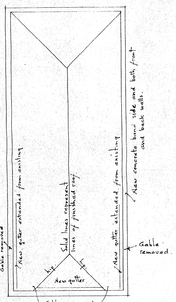
ROOF PLAN.
