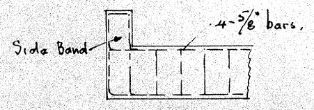
ELEVATION OF BACK BAND.
