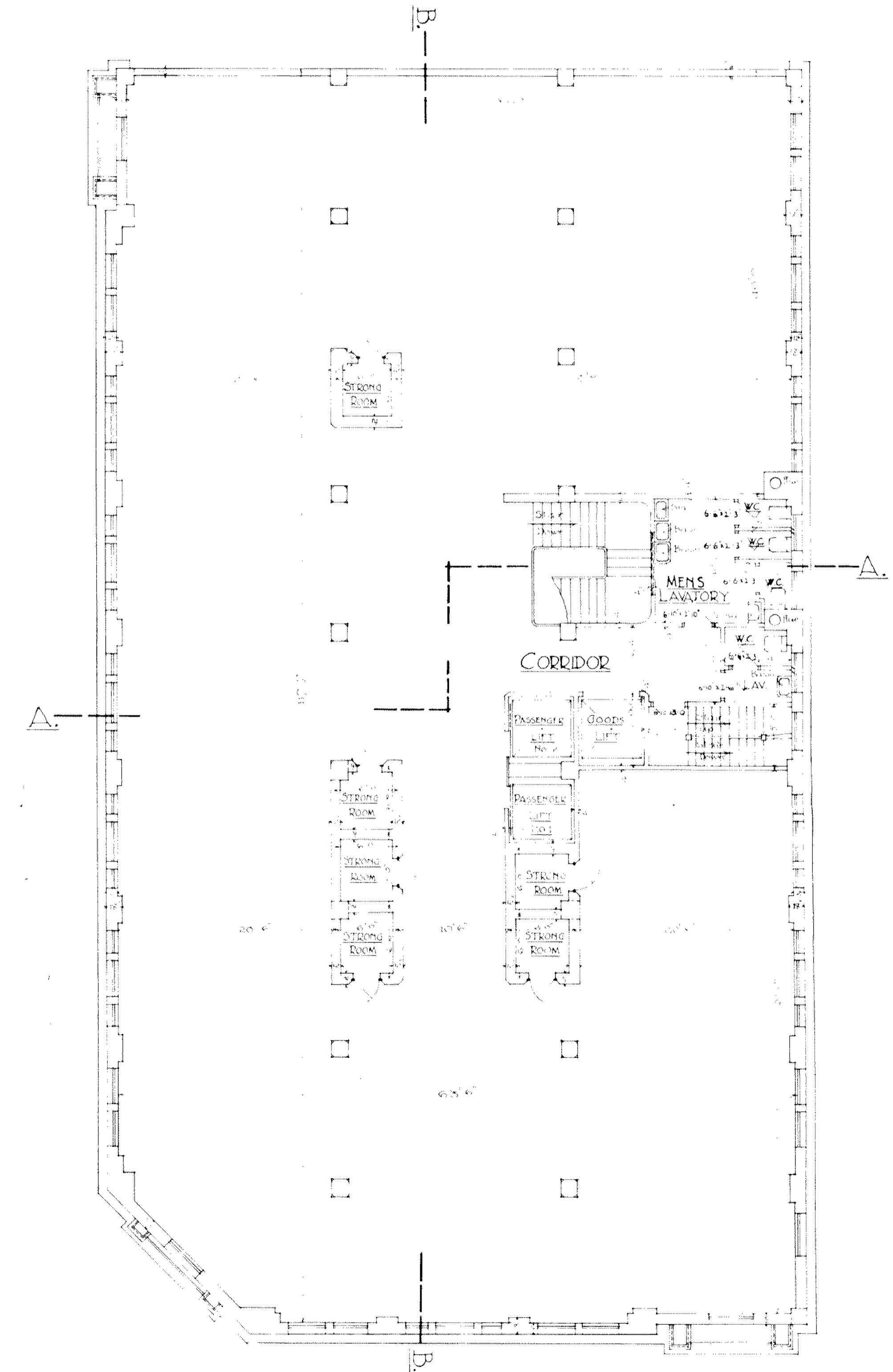
SIXTH FLOOR PLAN.
