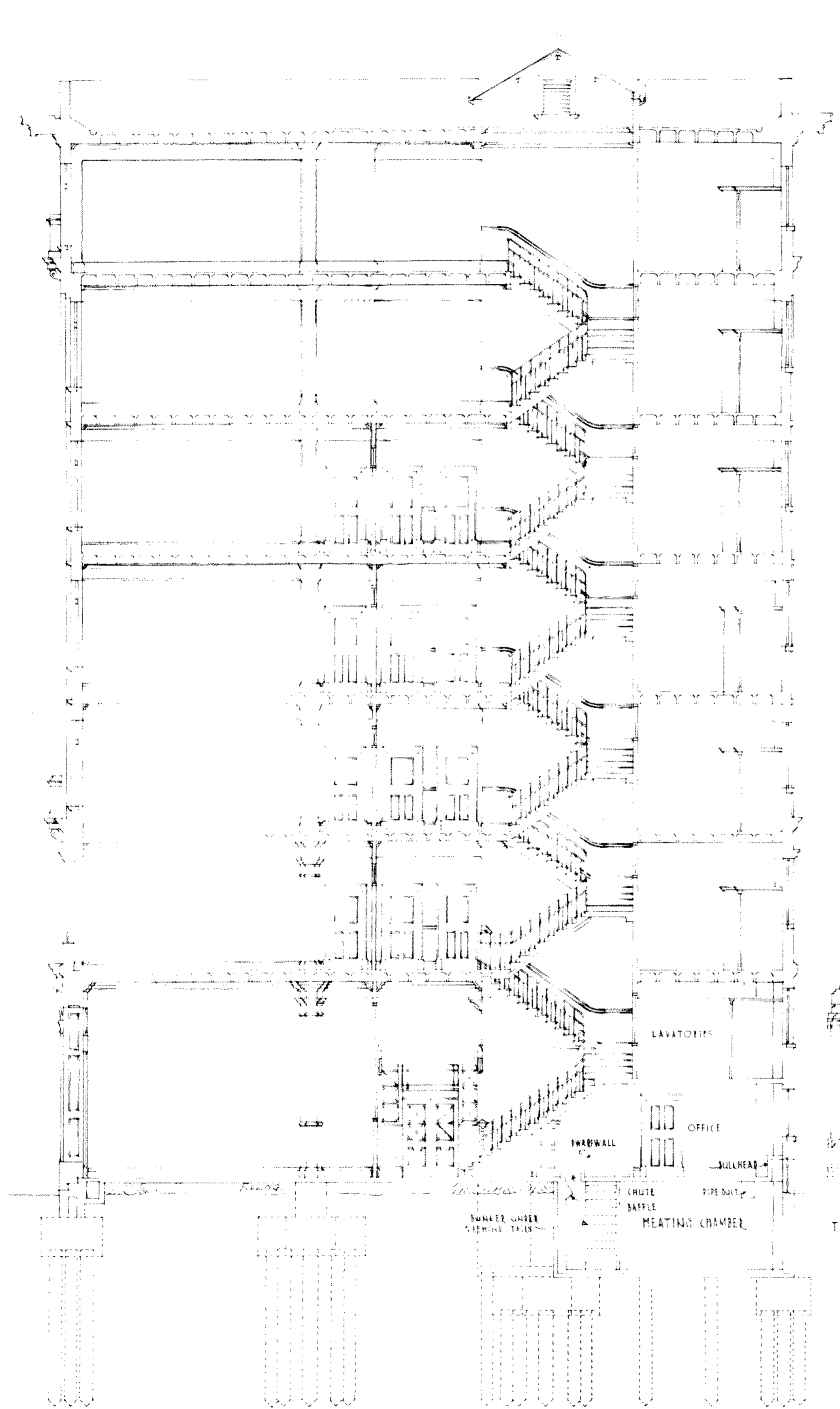
SECTION AA
