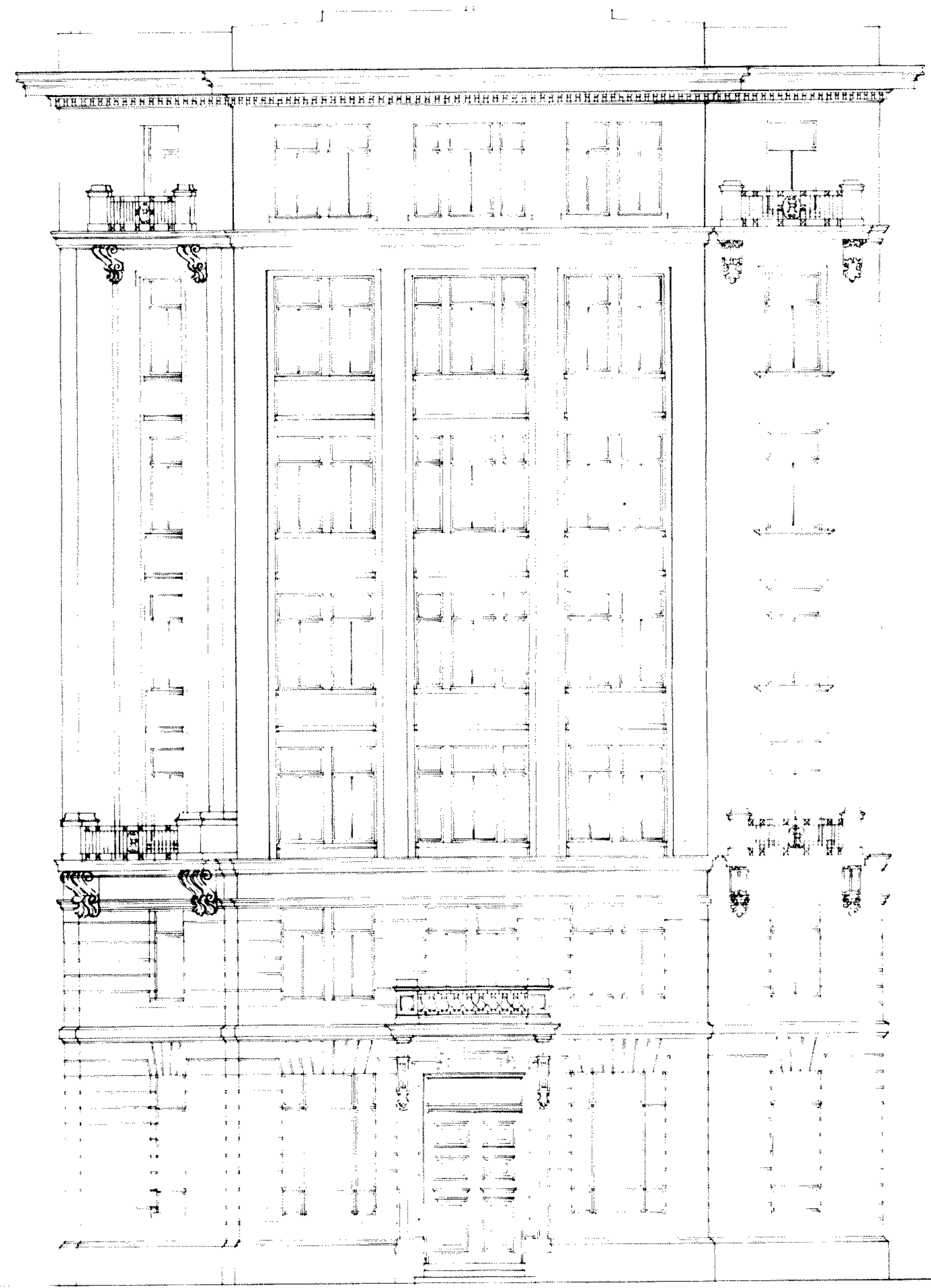
ELEVATION TO POST OFFICE SQUARE
