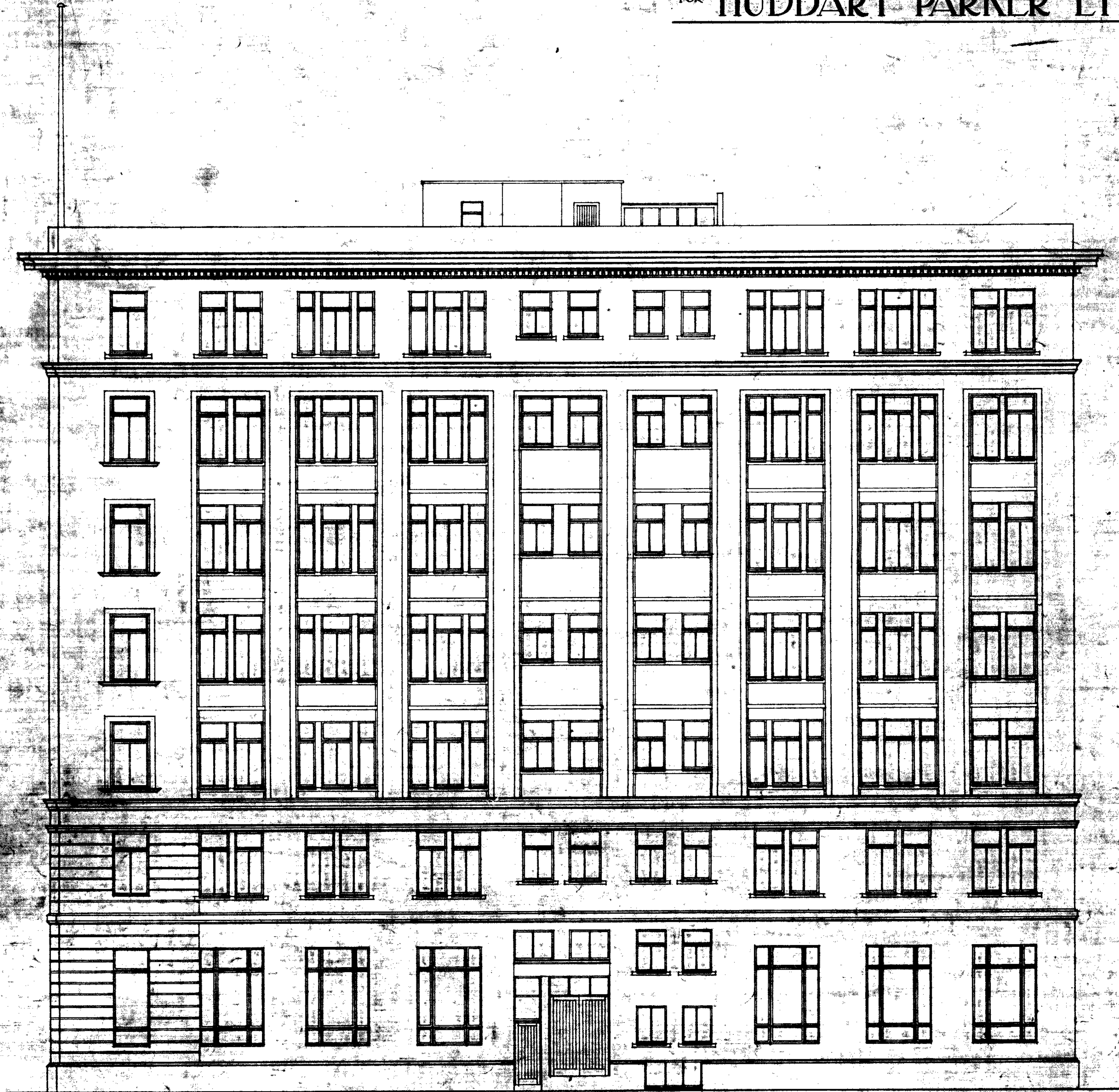
ELEVATION TO RESERVE
