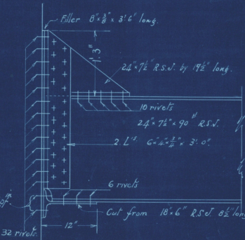
STRUCTURAL STEEL - TYPE 24 WK. DETAILS SCALE 1\"/>
