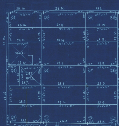
BEAMS & COLUMNS SUPPORTING SECOND FLOOR AND REAR ROOF :
