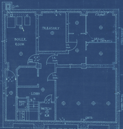
CEILINGS UNDER MEZZANINE FLOORS
