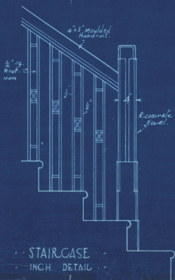
DETAIL OF R.C. STAIRCASE SCALE: \frac{1}{2} " = 1' WALL RODS NOT SHOWN
