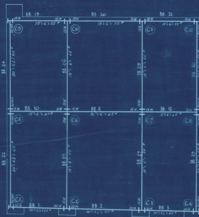
BEAMS & COLUMNS UNDER BASEMENT FLOOR
