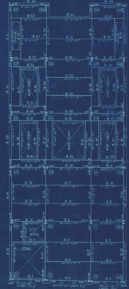
BEAMS & COLUMNS SUPPORTING FIRST FLOOR
