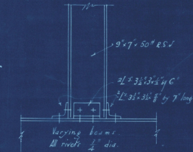
COLUMN DETAIL AT COLUMNS 25, 26, 27, 28, 29, 30, 31 & 32
