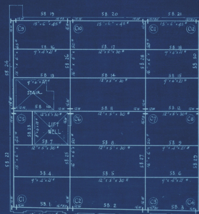
BEAMS & COLUMNS SUPPORTING FIFTH FLOOR :
