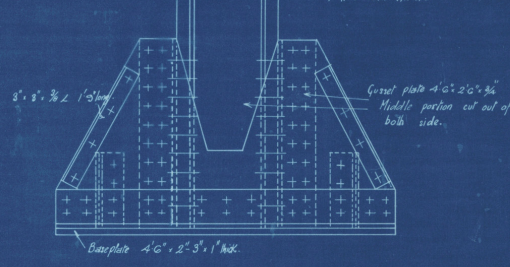
Plan and Elevation of Base to Columns 5, 6. TYPE (C)
