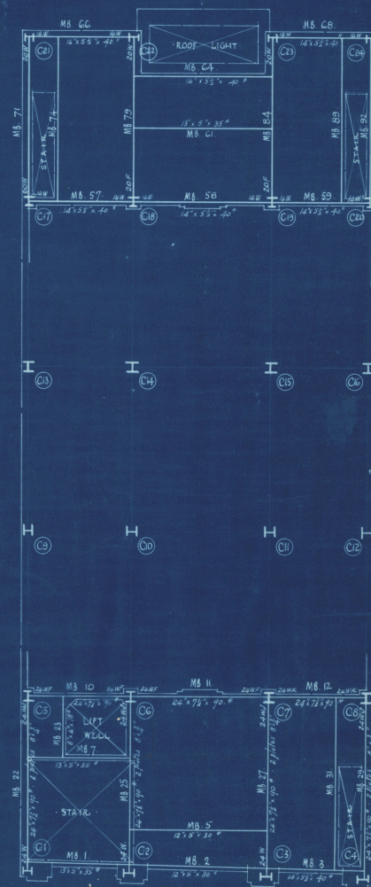
BEAMS & COLUMNS SUPPORTING MEZZANINE FLOOR
