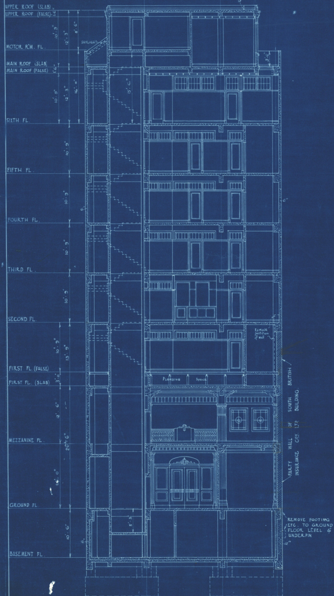
SECTION AT B · B
