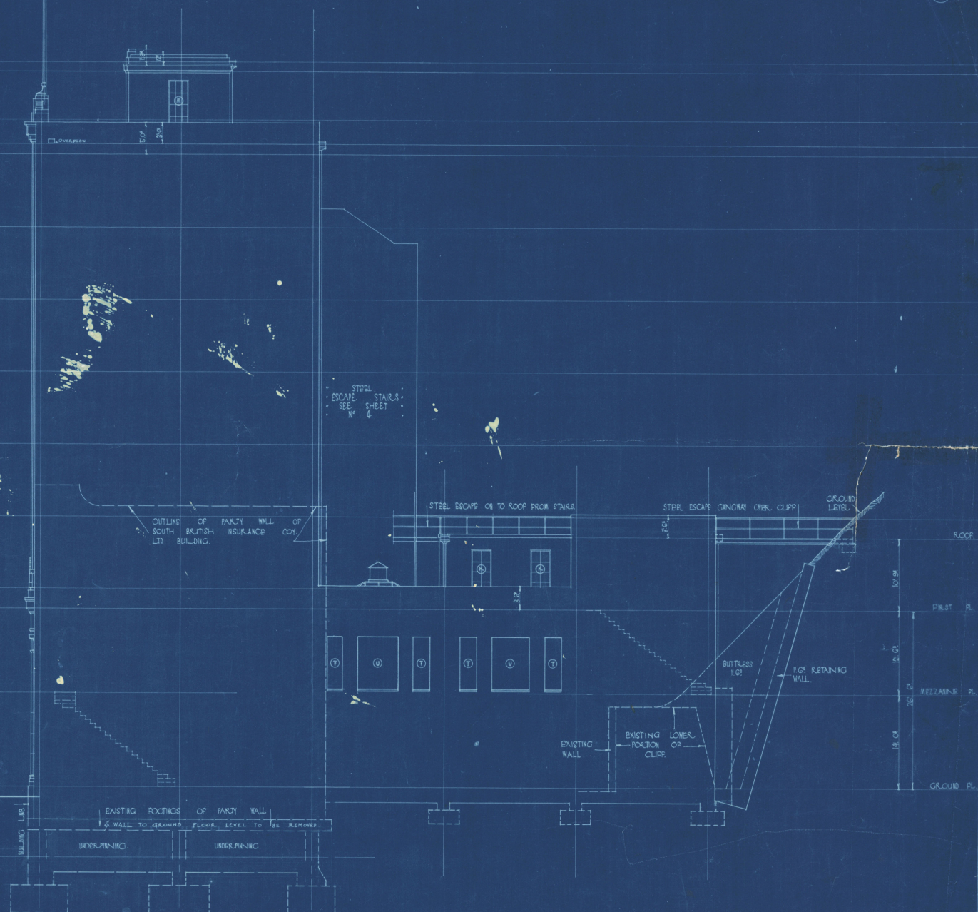
NORTH ELEVATION
