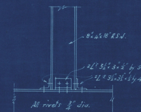
COLUMN DETAIL AT COLUMNS nos. 34, 35 & 36
