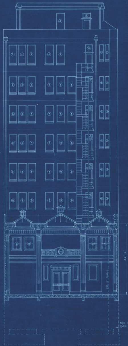
SECTION AT C · C
