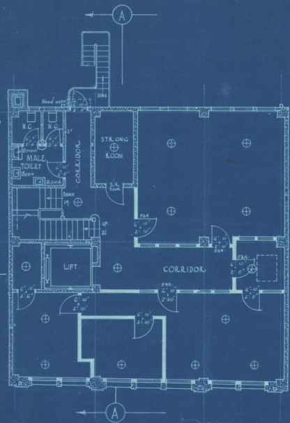
SIXTH FLOOR PLAN
