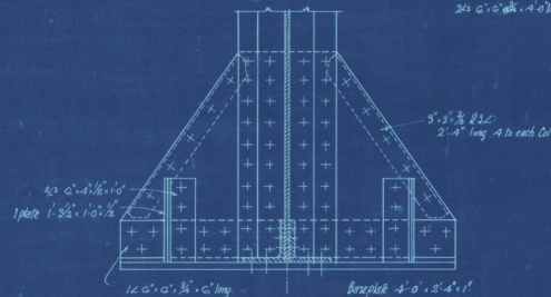
Plan and Section of Base to Cols. 1, 4, 9, 12. TYPE (A)
