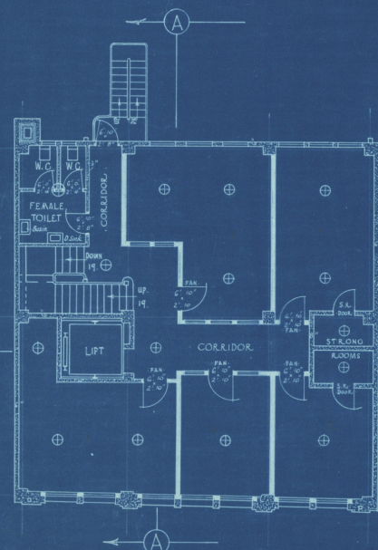
FIFTH FLOOR PLAN
