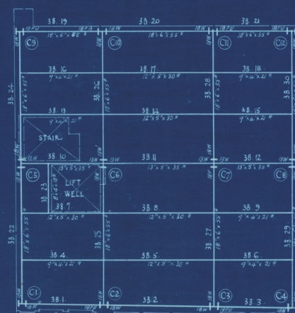
BEAMS & COLUMNS SUPPORTING THIRD FLOOR :
