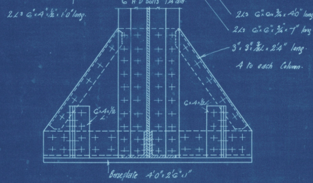
Plan and Section of Base Columns 2, 3, 10, 11. TYPE (B)
