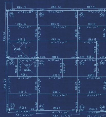
BEAMS & COLUMNS SUPPORTING MAIN ROOF :
