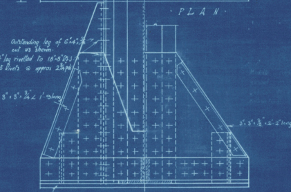
Half Elevation on 16" face of Stanchion. TYPE (E) COLS. 6, 7
