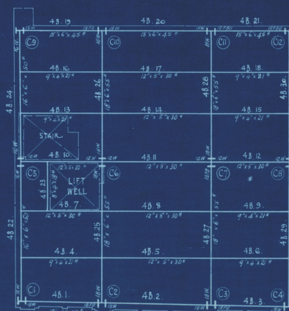
BEAMS & COLUMNS SUPPORTING FOURTH FLOOR :
