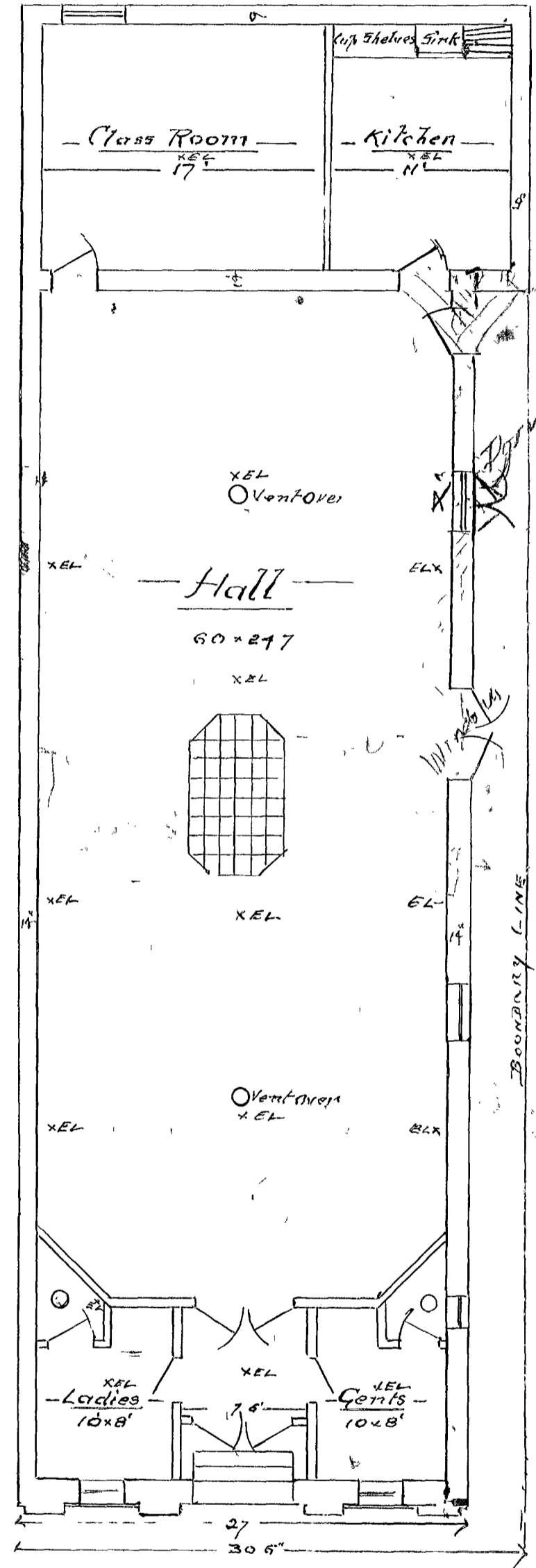
GROUND PLAN
