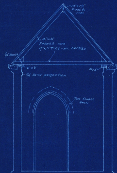
SECTION THRU PORCH LOOKING SOUTH SCALE 1/2" = 1 FOOT
