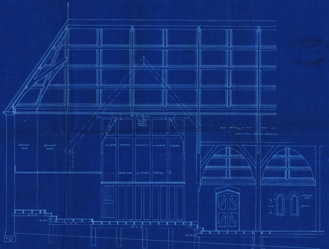
PART LONGITUDINAL SECTION LOOKING SOUTH
