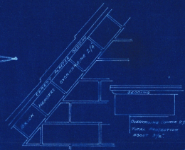
FINISH OF GABLES 1/16" TO FOOT
