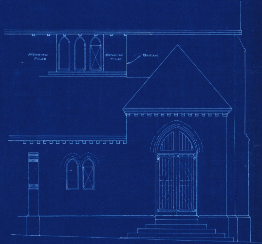
PART OF NORTH ELEVATION 1/4" = 1 FOOT
