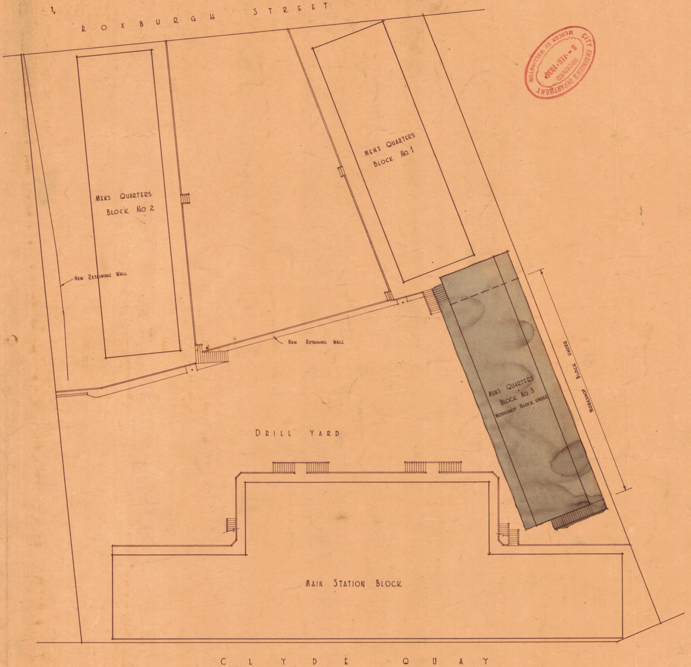
PLAN OF SITE SHOWING LAYOUT OF NEW BUILDINGS, WALLS, ETC. SCALE: 1/16" IN. = 1 FOOT
