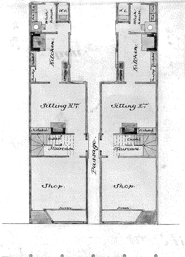
Ground Plan.
