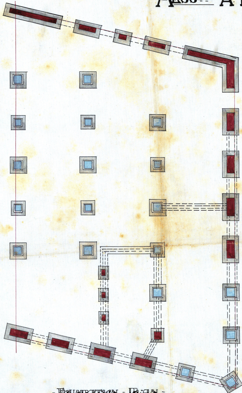
FOUNDATION PLAN
