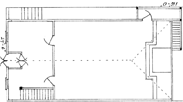
Ground Plan.
