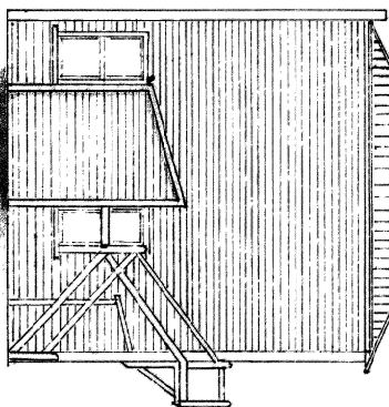
West Elevation.
